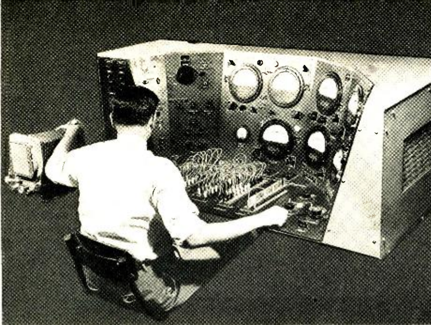
Console-type electronic tube characteristic curve tracer developed by Sylvania's Product Development Laboratories. Camera for photographing curves is at left.
