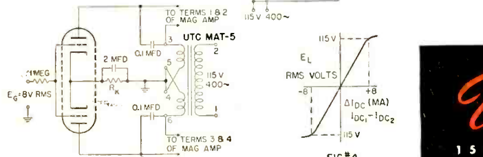
FIG #3 PARALLEL GRIDS-PUSH-PULL PLATES
