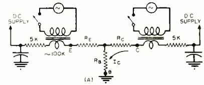
Fig. 1. Equivalent circuits for measuring (A) R_B and R_E , (B) \alpha , and (C) R_X .
