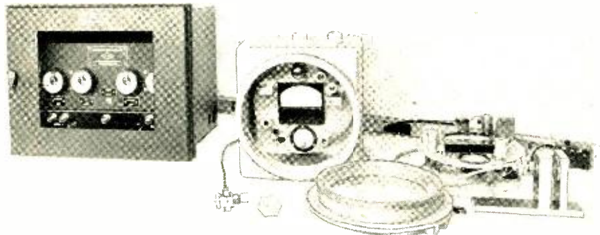
Shaft displacement indicator developed at NBS. Cabinet at left contains power supplies and alarm circuits. At center is the indicating unit and exciter unit, mounted in explosion-proof case for a special application. Transducer probe, in foreground, is the displacement-sensing element for this instrument. At right, exciter and indicator unit removed from case.
