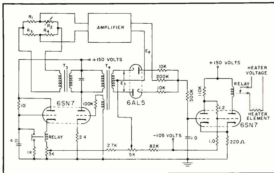
Schematic diagram of the time-proportional control circuit.
