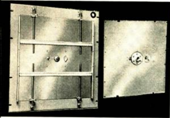
Fig. 6. Open view of the sweep cavity.
