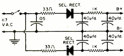
Fig. 3. Schematic of a power supply suitable for use with Figs. 1 and 2.
