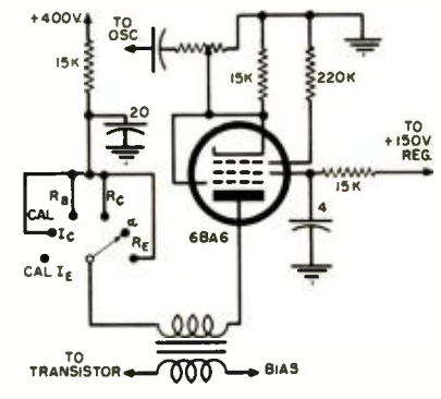
Fig. 5. Collector signal supply circuit.
