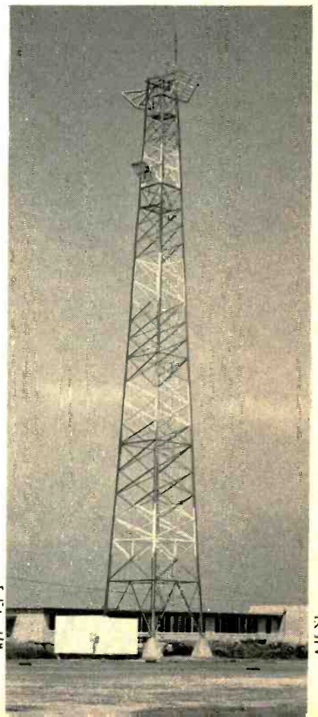
Tower at Port Sulphur. Lower reflector faces toward Grande Ecaille.
